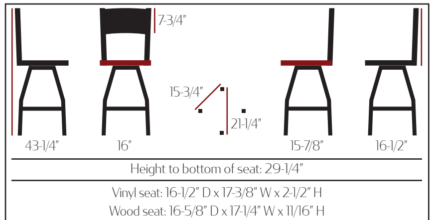
Clear Coat Wood Back & Espresso Vinyl Seat SL2150-IS-P-N-ESP
