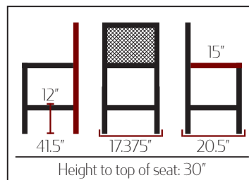
Two-Piece Assembly
